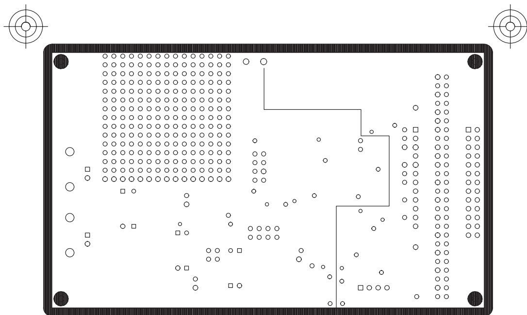
Figure 2–2. PCB Layout
