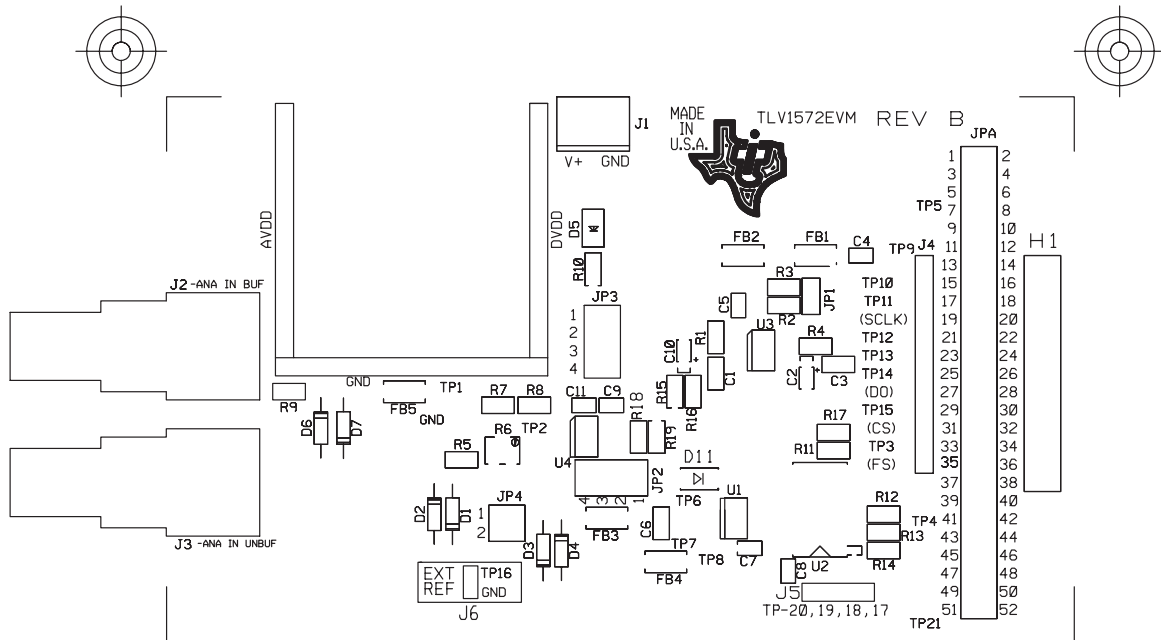
Figure 2–5. PCB Layout
