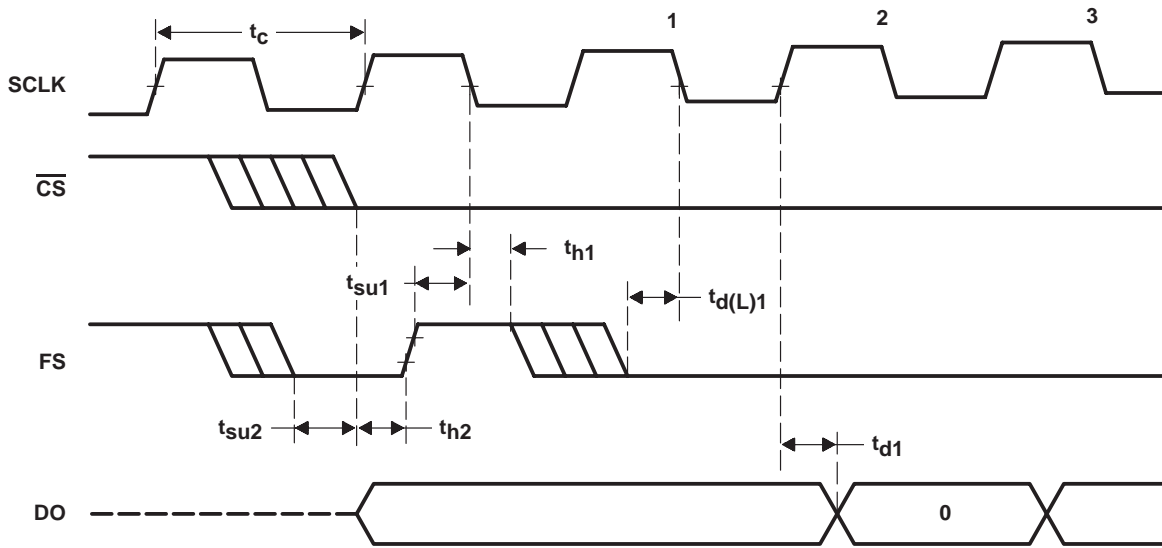
Figure 4–2. Microprocessor Interface Timing (Normal Sample Mode, \overline{INV\ CLK} = \text{High} )
