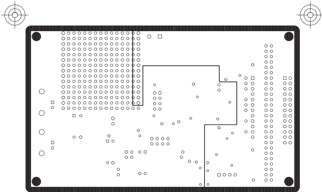
Figure 2–3. PCB Layout
