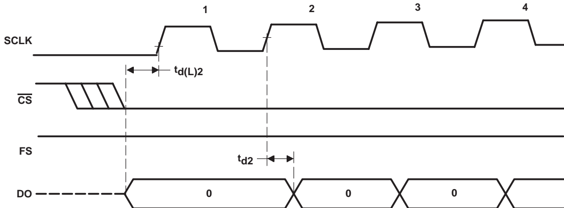
Figure 4–3. Microprocessor Interface Timing (Normal Sample Mode, \overline{INV\ CLK} = \text{Low} )
