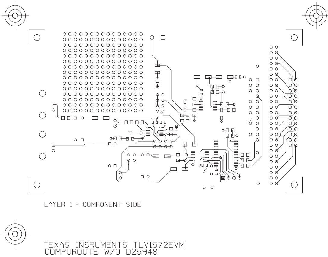
Figure 2–1. PCB Layout
