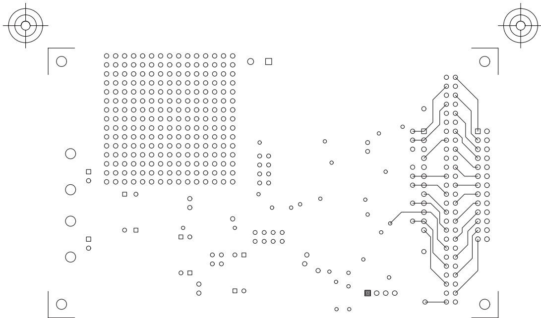
Figure 2-4. PCB Layout
